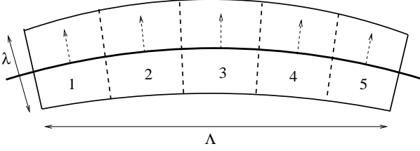
Fig. 2.6. Sector K_{\Lambda, \lambda}^{\alpha} on the Fermi surface (thick solid line) with non-negligible curvature. The dashed arrows are the local normal vectors at the Fermi surface. The dashed lines separate the smaller boxes which are more appropriate if the energy dispersion is linearized. Note that around-the-corner processes corresponding to momentum transfer between the smaller boxes 1 \leftrightarrow 2 , 2 \leftrightarrow 3 , 3 \leftrightarrow 4 and 4 \leftrightarrow 5 are automatically taken into account in K_{\Lambda, \lambda}^{\alpha} .
