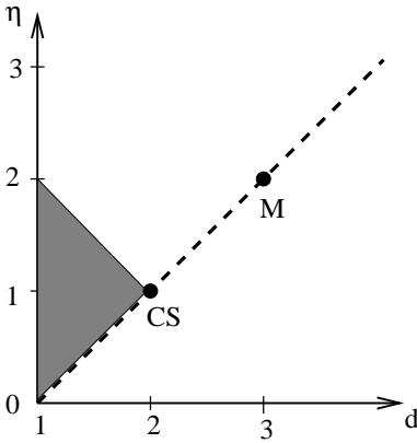
Fig. 10.3. The shaded triangle is the parameter regime in the d - \eta -plane where the long-distance and large-time behavior of the Debye-Waller Q_{\text{tr}}^{\alpha}(r_{\parallel}^{\alpha} \hat{\nu}^{\alpha}, \tau) due to transverse gauge fields gives rise to non-Fermi liquid behavior. Note that for linearized energy dispersion one incorrectly obtains non-Fermi liquid behavior for all points above the dashed line \eta = d - 1 . The points M and CS correspond to the three-dimensional Maxwell theory and the two-dimensional Maxwell-Chern-Simons theory, respectively.
